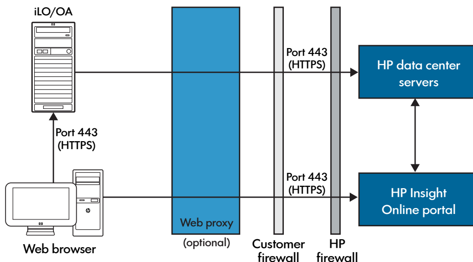
Figure 3 Network requirements for Insight Online direct connect
